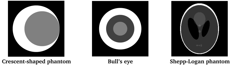
Figure 4: Three popular phantoms. Crested-shaped phantom, bull's eye, and Shepp-Logan (each of size 256 \times 256 ).
