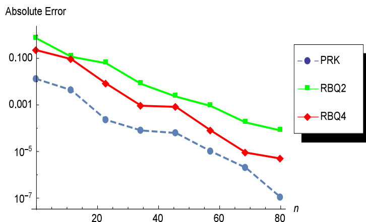
Figure 1: The absolute error of PRK and BRQ solutions for the Example 7.2
