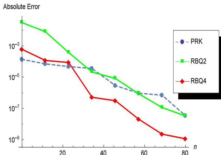
Figure 1: The absolute error of PRK and BRQ solutions for the Example 7.2
