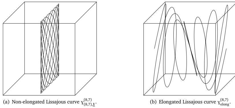
Figure 4: Example illustration of the Lissajous curve v_{(8,7),1}^{(8,7)} in non-elongated and elongated form.
